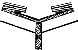
Section of Valley on M.M.
